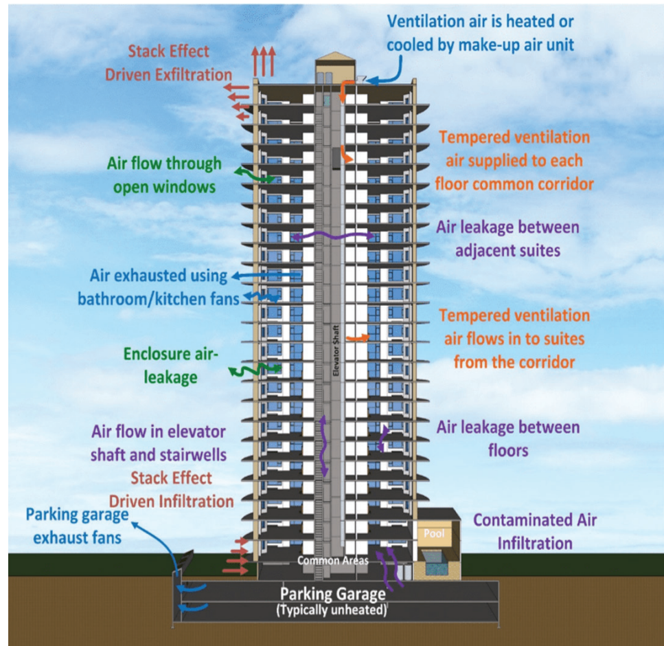
Figure 5-2. High-rise Building Section Showing Stack Ventilation
