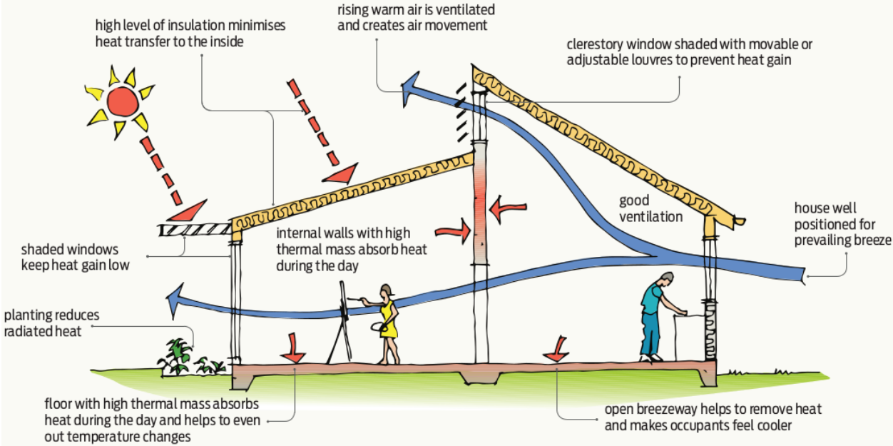
Figure 5-9. Overall Passive Design Strategies (Source: Archi monarch -2023 https://archi-monarch.com/ )
