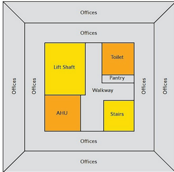
Figure 5-6. Square Building Centre Core
