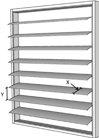
Figure 4-3: Horizontal Louvres (Relationship between depth (x) and gap (y): x \geq 0.234y )
