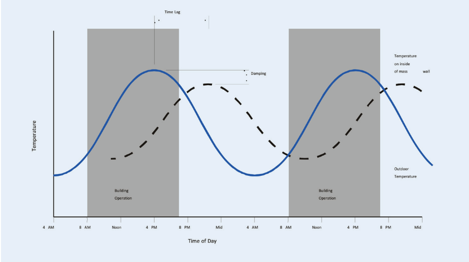
Figure 7-2. Temperature Swing
