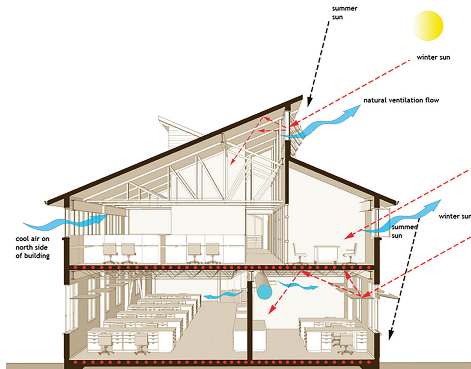
Figure 5-1. Building Section Showing Cross Ventilation
