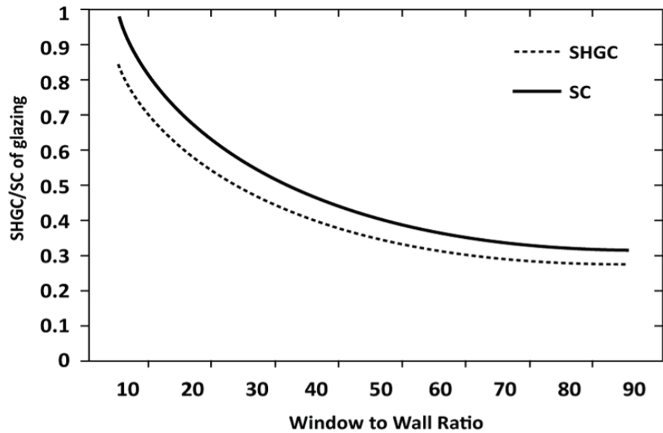
Figure 4-1. Selection of Glazing SHGC Based on WWR
