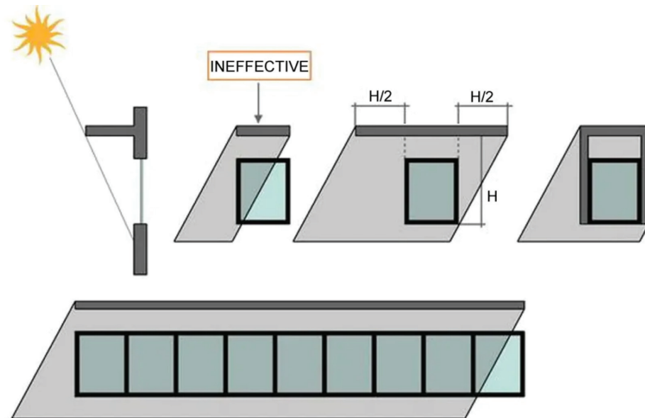
Figure 5-5. Façade Design with External Shading
