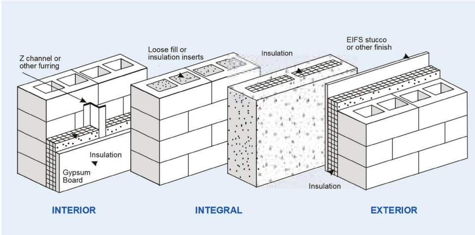
Figure 7-3. Construction of Mass Walls of Buildings
