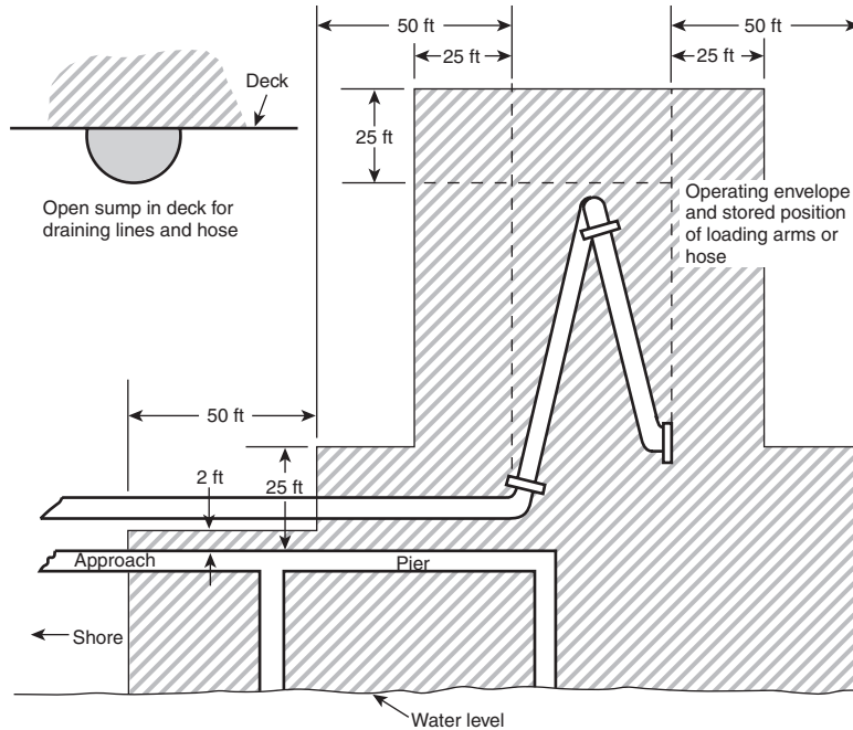
Figure 515.3 Marine Terminal Handling Flammable Liquids. [30:Figure 29.3.22]
