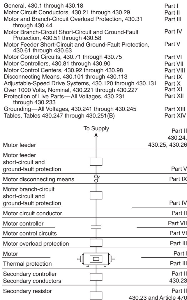
Figure 430.1 Article 430 Contents.
