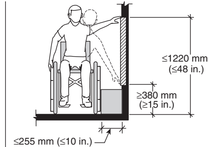
Figure J.7.1 Unobstructed Side Reach.
