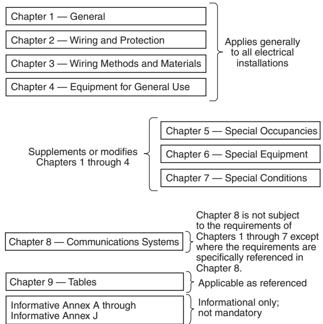
Figure 90.3 Code Arrangement.
