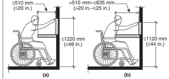
Figure J.6.2 Obstructed High Forward Reach.
