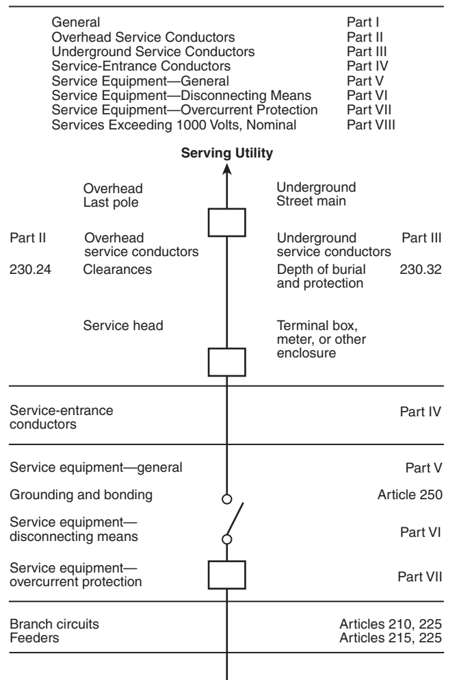
Figure 230.1 Services.
