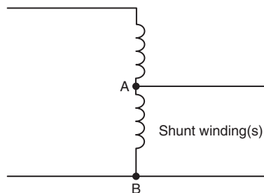
Figure 450.4(A) Autotransformer.
