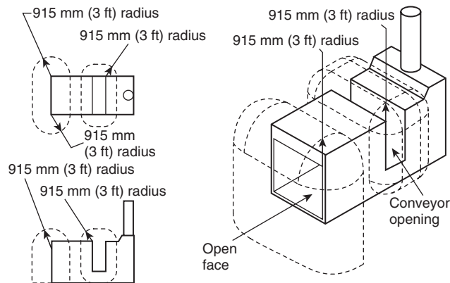
Figure 516.3(D)(2) Class I, Division 2; Class I, Zone 2; Class II, Division 2; or Zone 22 Locations Adjacent to a Closed Top, Open Face, or Open Front Spray Booth or Room.
