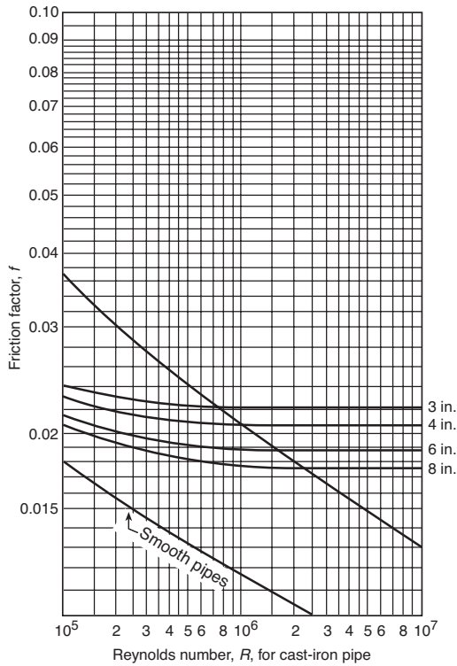
FIGURE 7.4.1.4.1(b) Moody Diagram for Cast-Iron Pipe, R \geq 10^5 .
