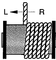
Start rope at right hand flange for right hand lay rope.
