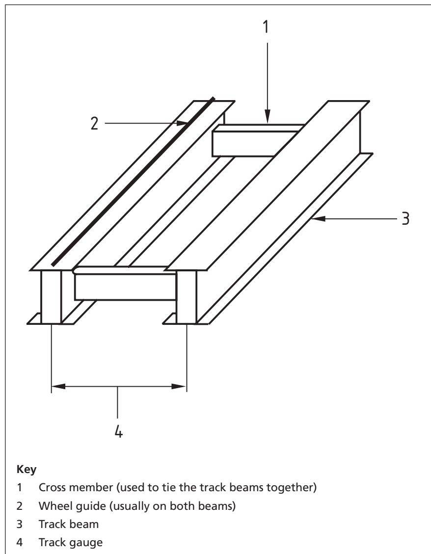
Figure 3 Track beams
