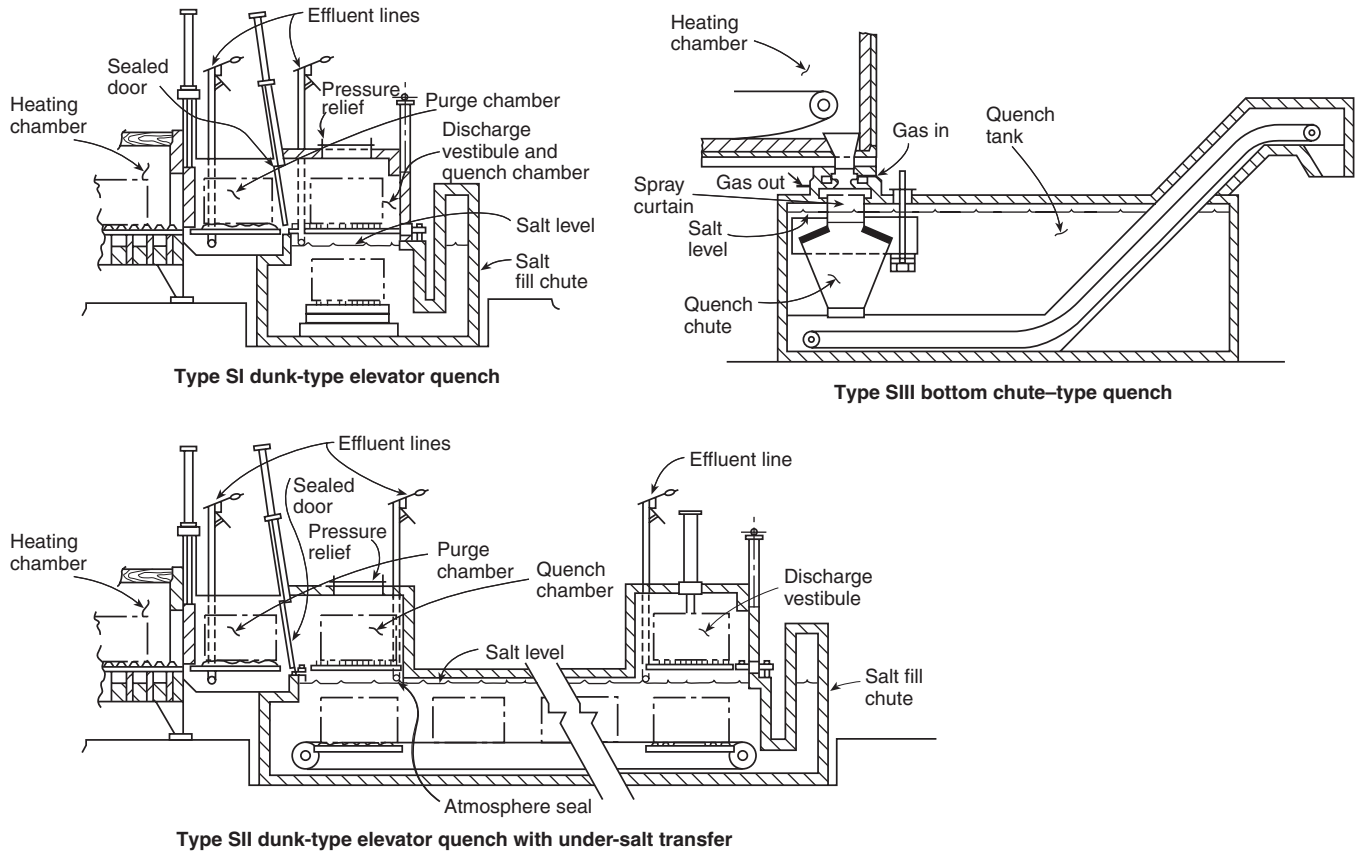
FIGURE A.13.5.15.6.1 Examples of Integral Quench Tanks.
