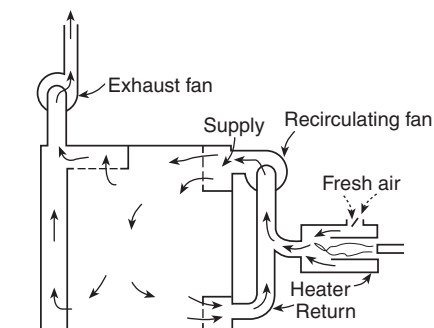
FIGURE A.3.3.33.3(c) Example of a Direct-Fired, External, Recirculating-Not-Through Heater.
