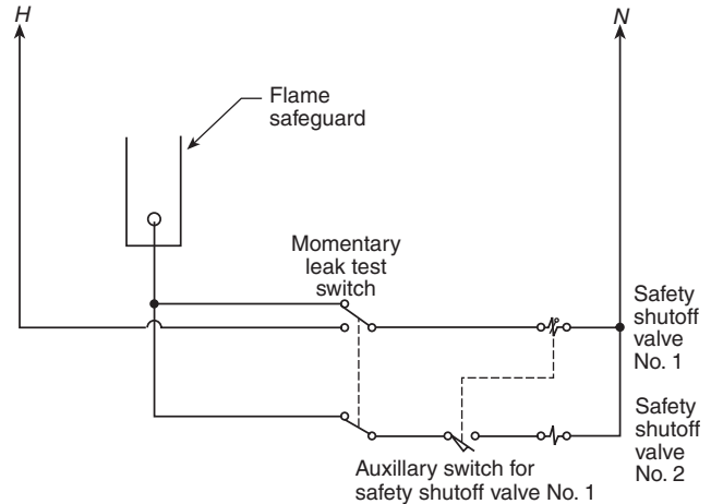
FIGURE A.7.4.9(b) Example of a Wiring Diagram for Leak Test.
