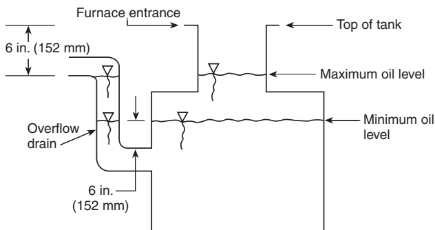
FIGURE A.13.5.13.5(E) Example of Overflow Drains for Closed Integral Quench Tanks.
