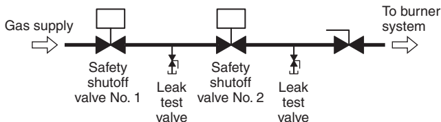
FIGURE A.7.4.9(a) Example of a Gas Piping Diagram for Leak Test.
