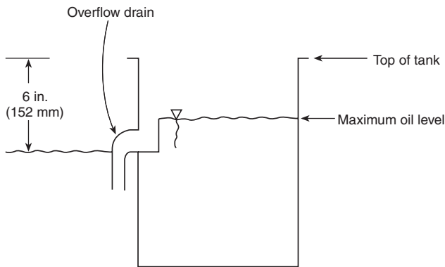
FIGURE A.13.5.13.5(D) Example of Overflow Drains for Open Integral Quench Tanks.
