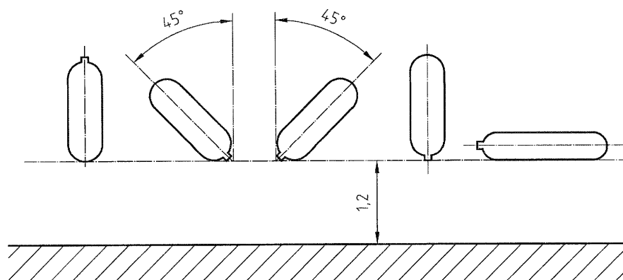
Figure 1 — Drop test
